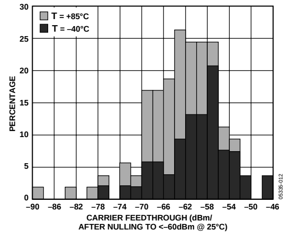
Figure 12. Histogram Showing Carrier Feedthrough Distributions at the Temperature Extremes after Nulling at Ambient at F_{LO} = 1900\text{ MHz} , LO Input Level = -10 dBm.
