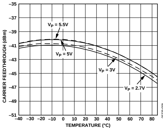
Figure 9. Carrier Feedthrough vs. Temperature. F_{LO} = 1900\text{ MHz} , LO input level = -10 dBm.
