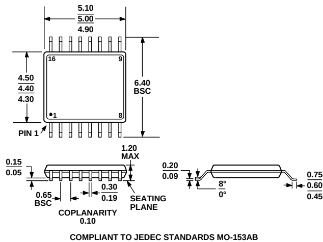
Figure 37. 16-Lead Thin Shrink Small Outline Package [TSSOP] (RU-16) Dimensions shown in millimeters
