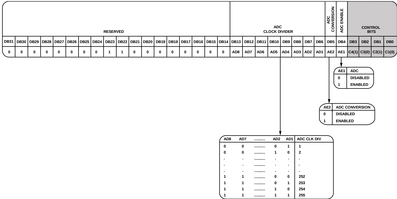
Figure 48. Register 10 Details
