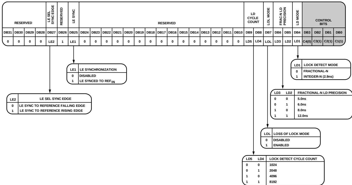
Figure 45. Register 7 Details
