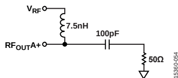
Figure 54. Optimum Output Stage
