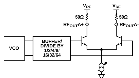
Figure 34. Output Stage
