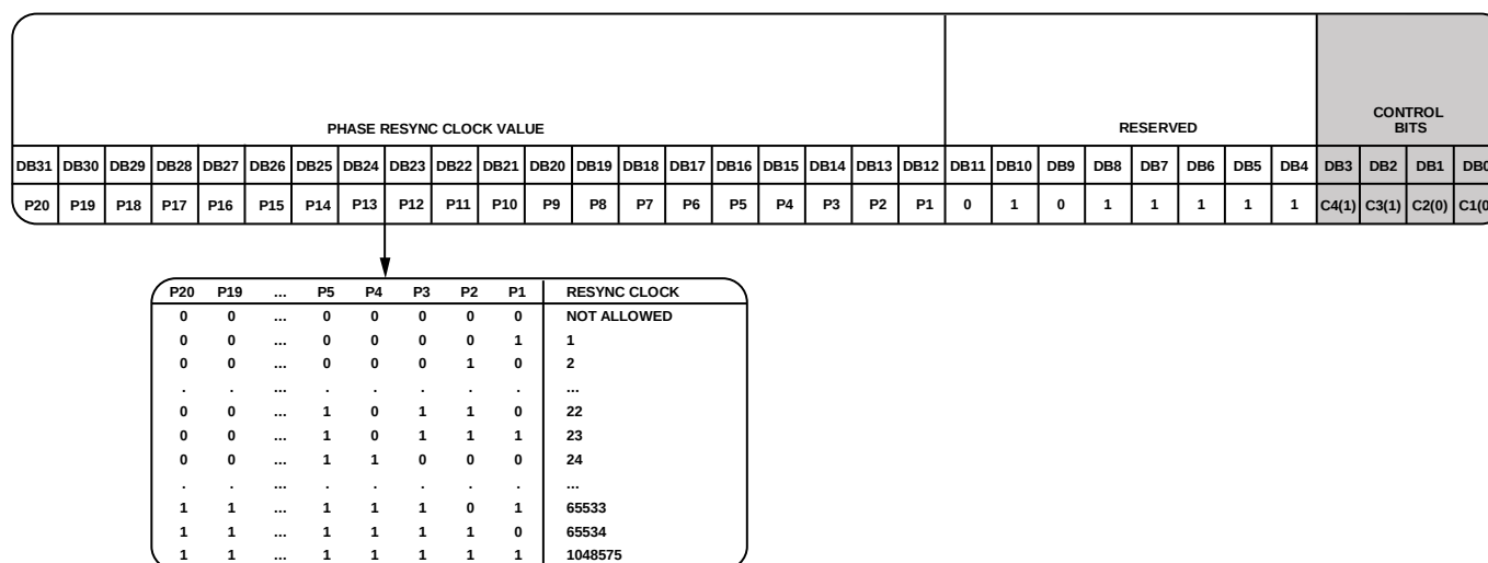
Figure 50. Register 12 Details
