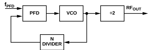
Figure 52. Loop Closed Before Output Divider
