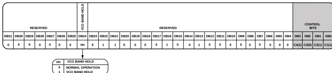
Figure 49. Register 11 Details
