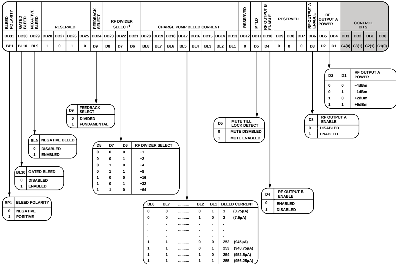
Figure 44. Register 6 Details
