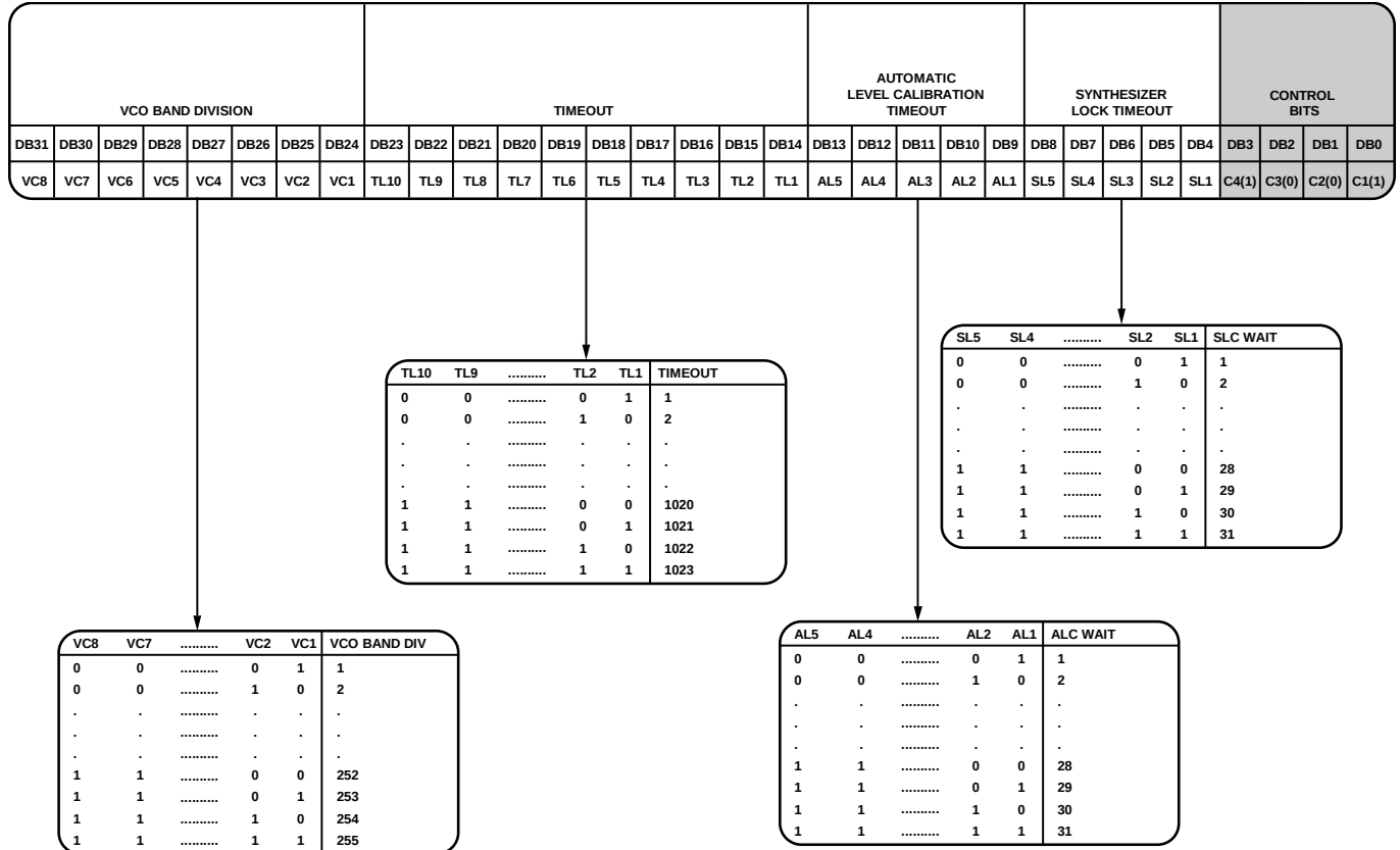
Figure 47. Register 9 Details
