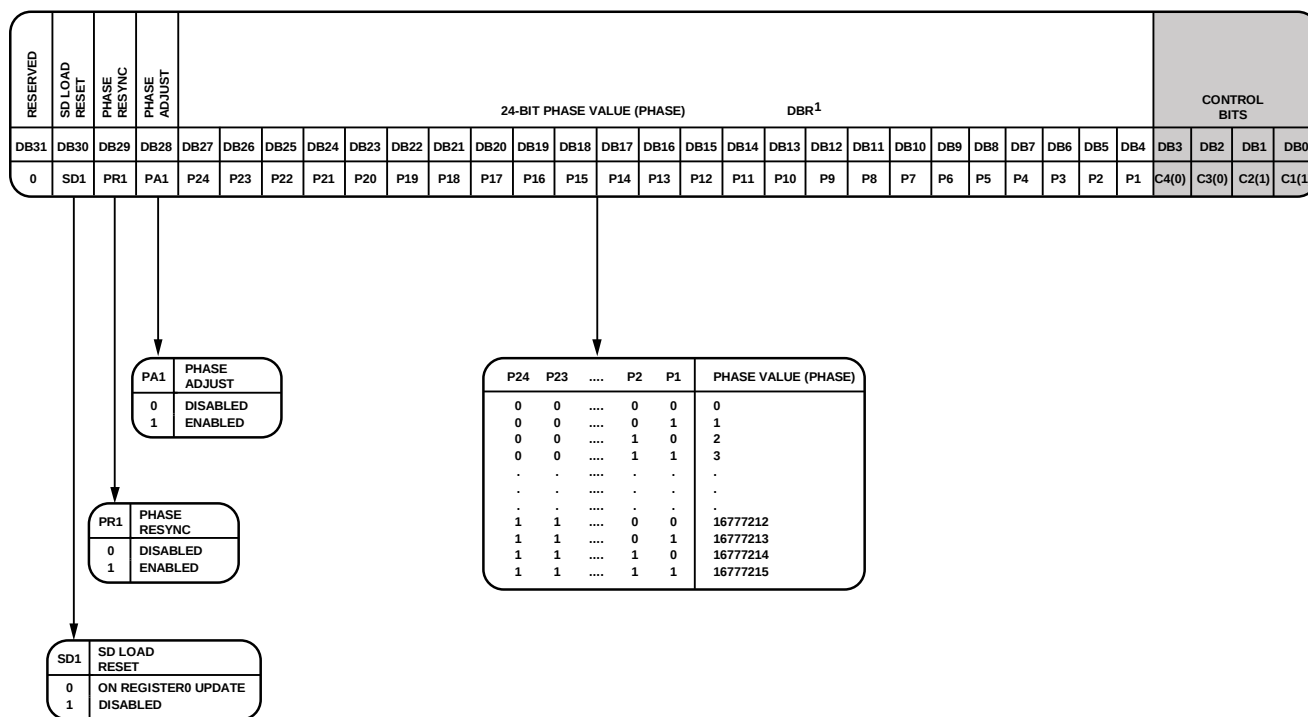
Figure 41. Register 3
