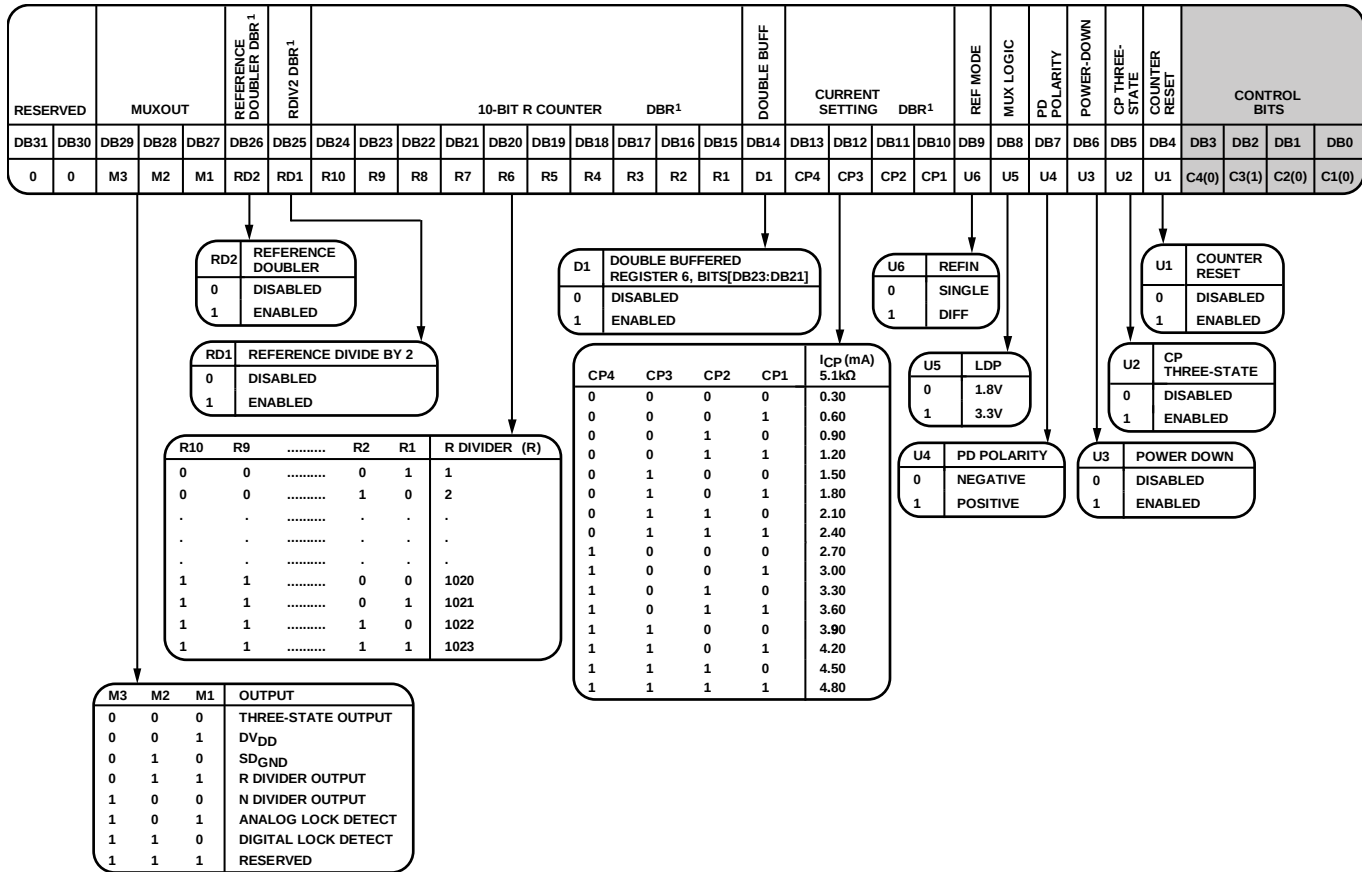
Figure 42. Register 4 Details
