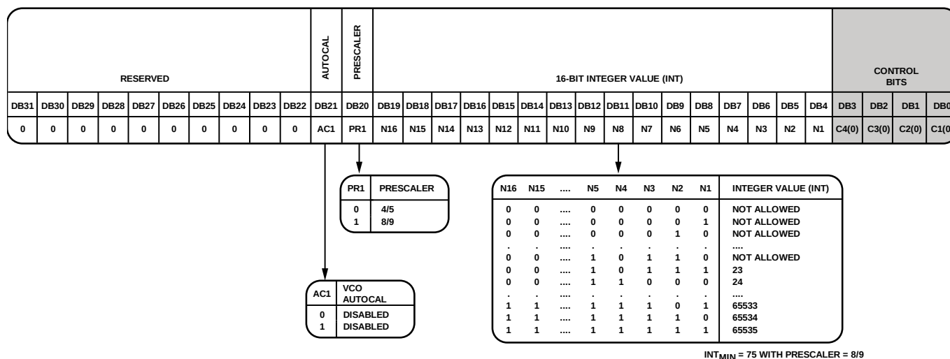
Figure 38. Register 0 Details
