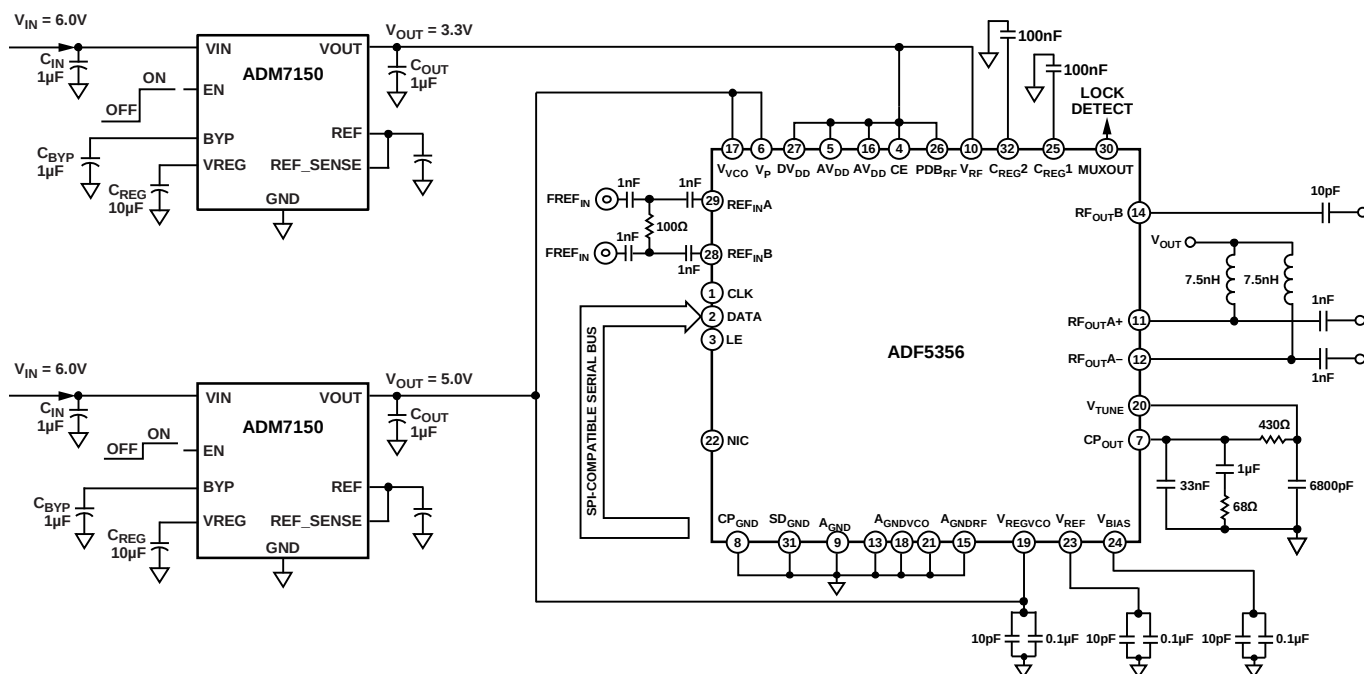
Figure 53. Power Supplies
