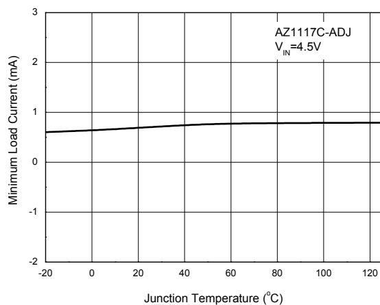
Figure 8. Minimum Load Current vs. Junction Temperature
