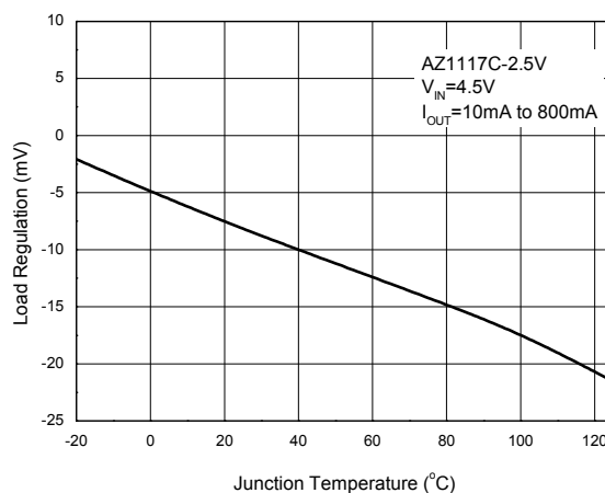
Figure 5. Load Regulation vs. Junction Temperature
