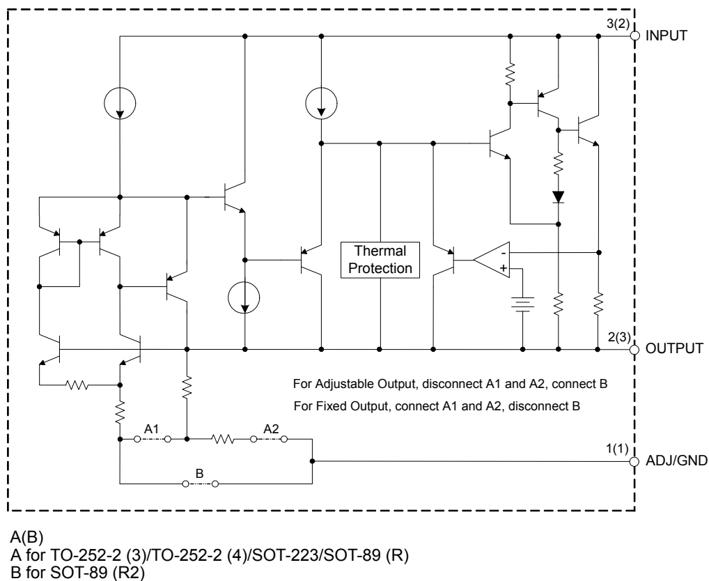
Figure 3. Functional Block Diagram of AZ1117C
