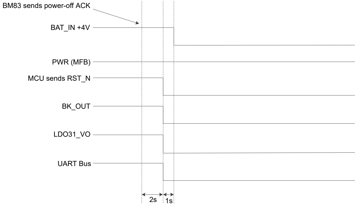
Figure 6-4. Timing Sequence of Power-OFF State
