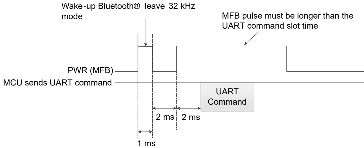
Figure 6-4. Timing Sequence of Power-OFF State
