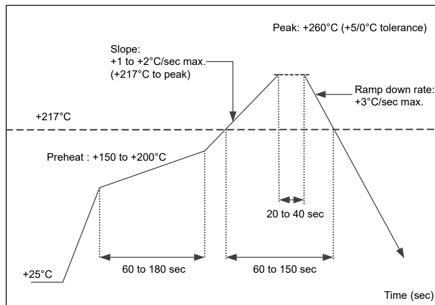
Figure 10-1. Reflow Profile
