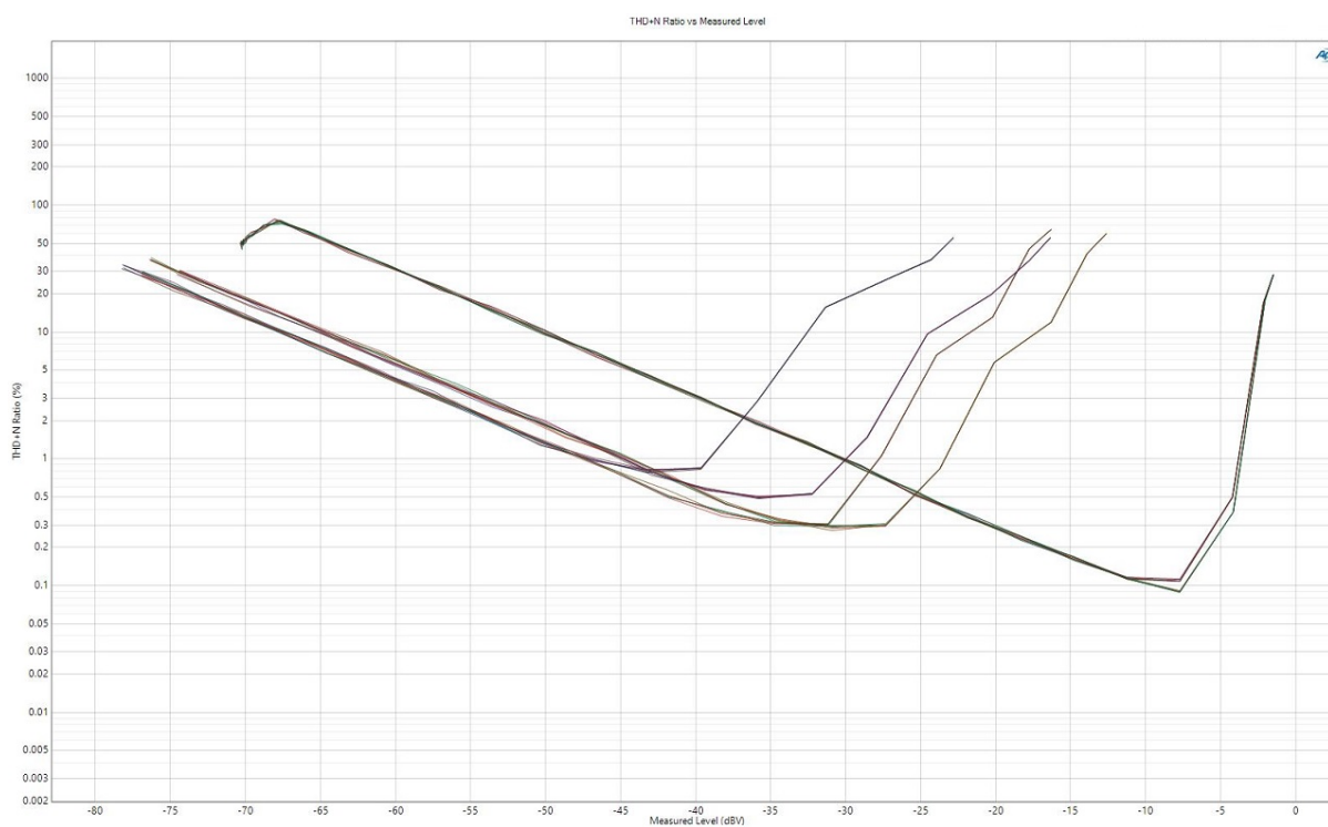
Figure 3-18. THD+N Ratio (%) Vs. Output Level at Various Loads (Single-ended mode)
