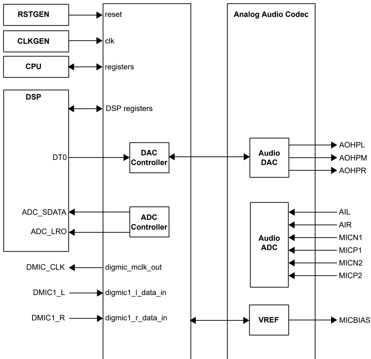
Figure 3-1. Audio Subsystem
