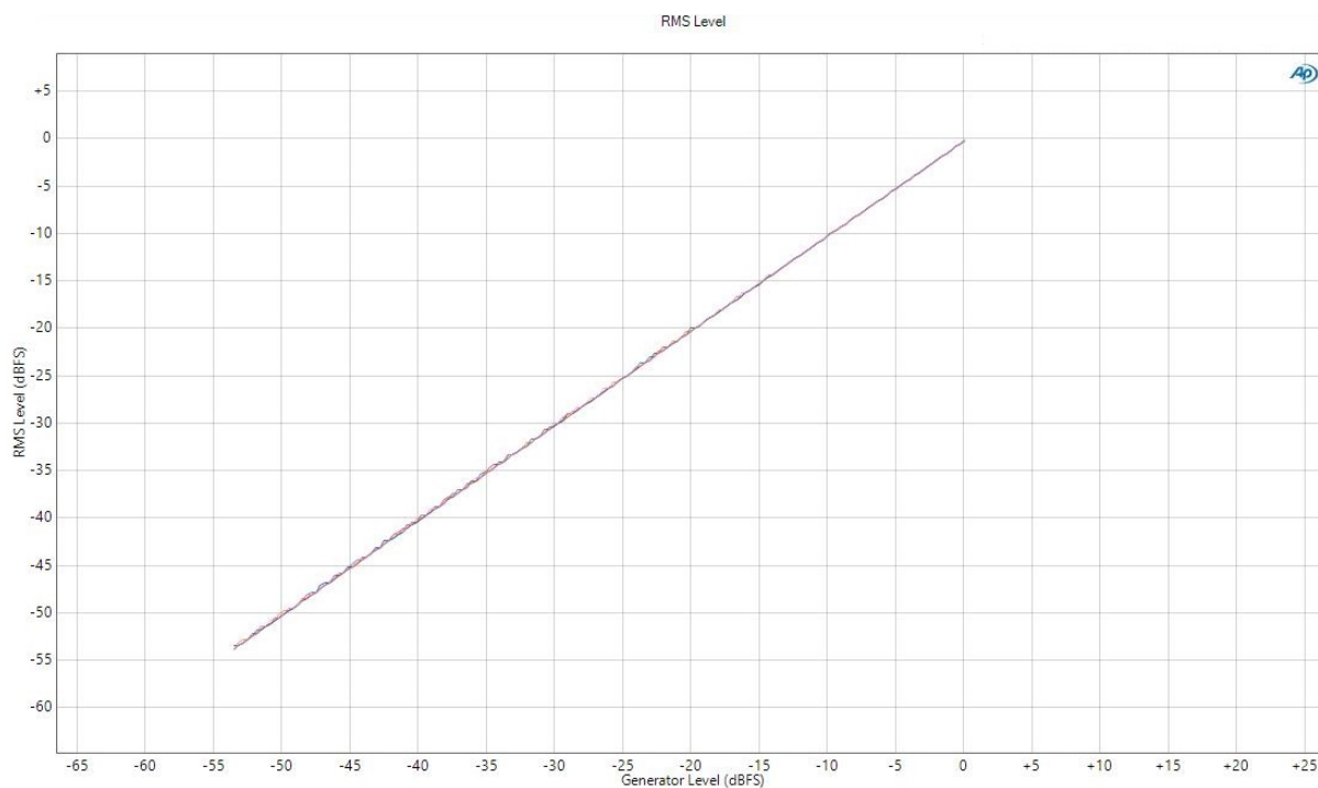
Figure 3-22. Output Level Vs. Input Level
