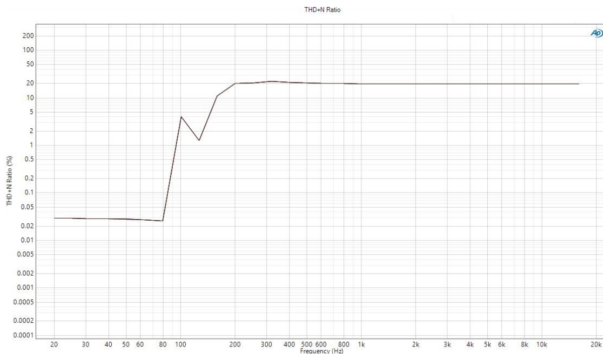
Figure 3-28. THD+N Ratio (%) Vs. Frequency
