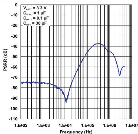
Figure 6. Power Supply Rejection vs Input Frequency
