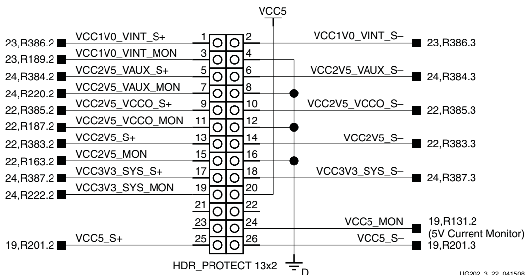
Figure 3-21: P72 Pinout Diagram (Sheet 20)
