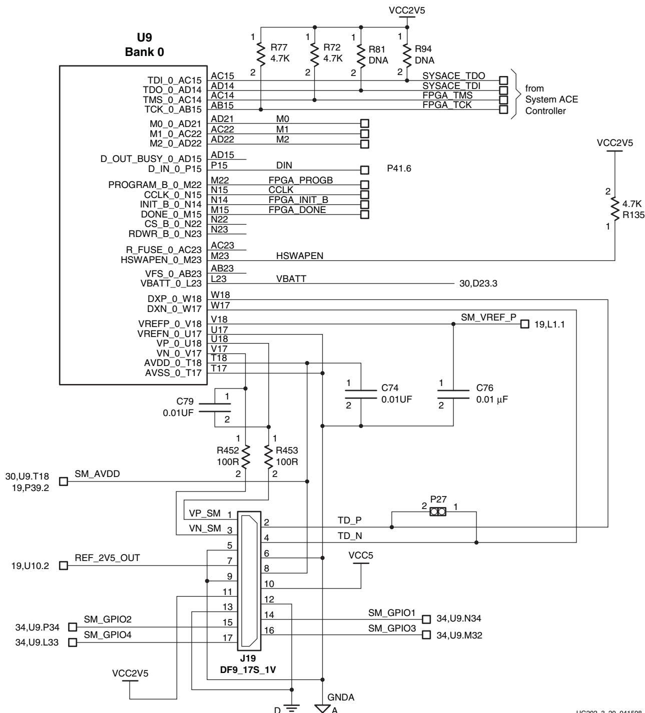
Figure 3-20: J19 Mezzanine Board Connector (Sheet 30)
