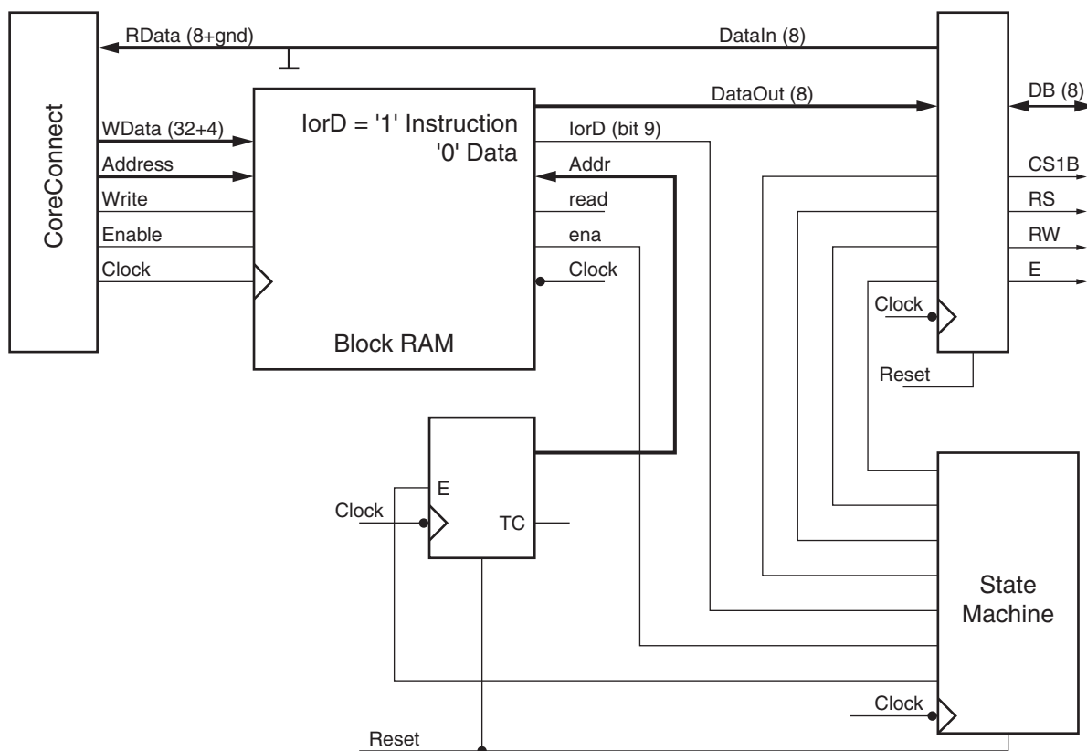
Figure C-8: General Block Diagram of Panel in Full Graphics Mode
