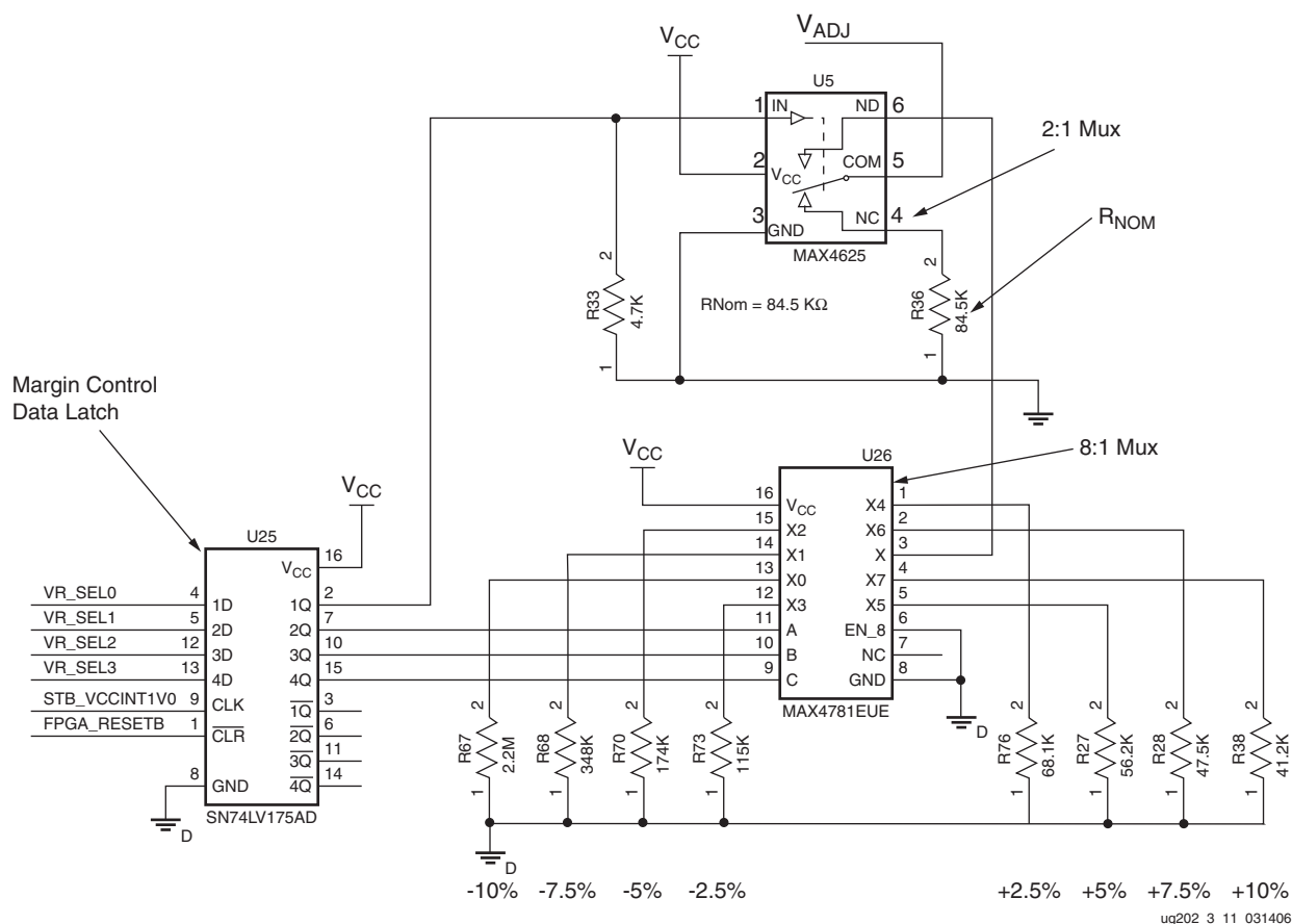
Figure 3-9: Margin Control Circuit Details
