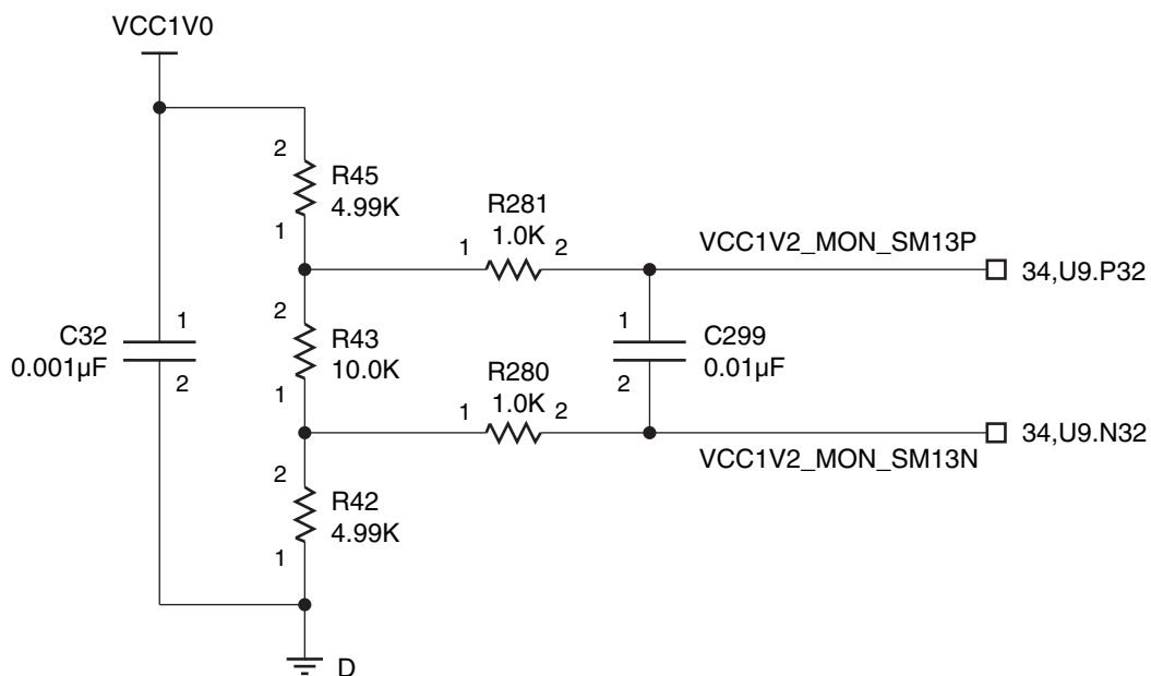
Figure 3-16: 1.0V V_{CCINT} Voltage Monitor (Sheet 20)
