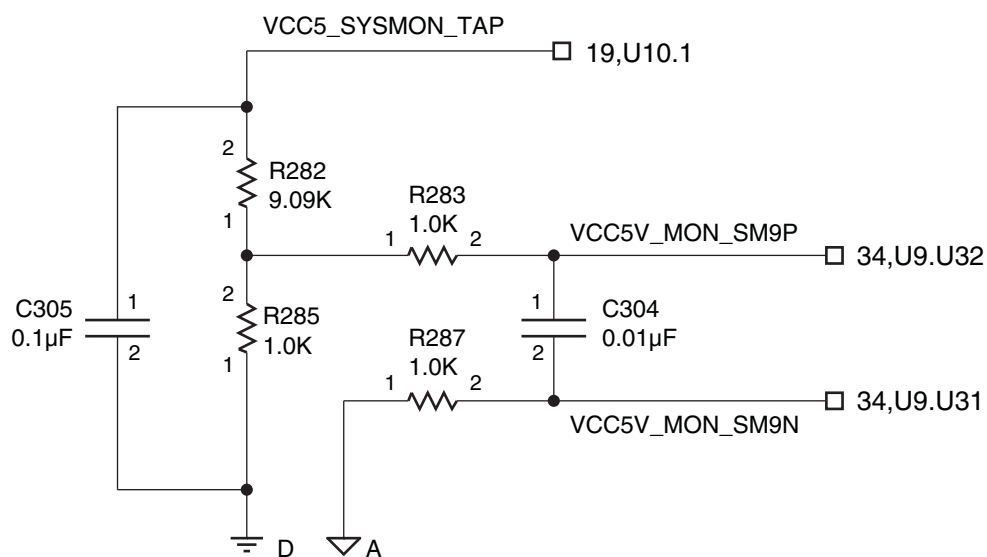
Figure 3-12: 5V Input Power Voltage Monitor (Sheet 19)
