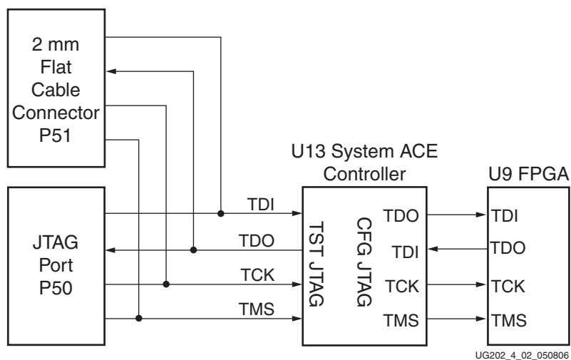
Figure 4-2: JTAG Chain
