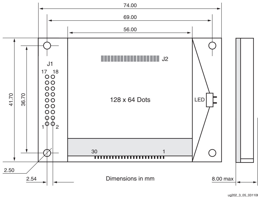
Figure 3-5: 64128EFCBC-3LP Dimensions
