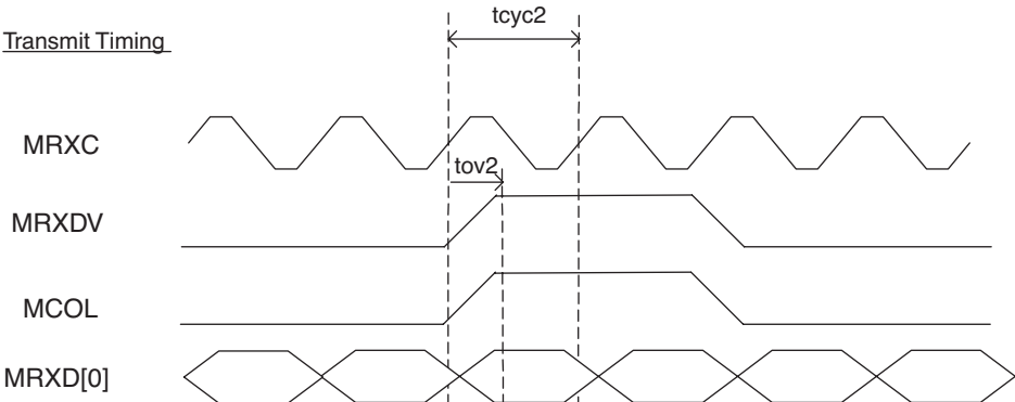
Figure 15. SNI Output Timing
