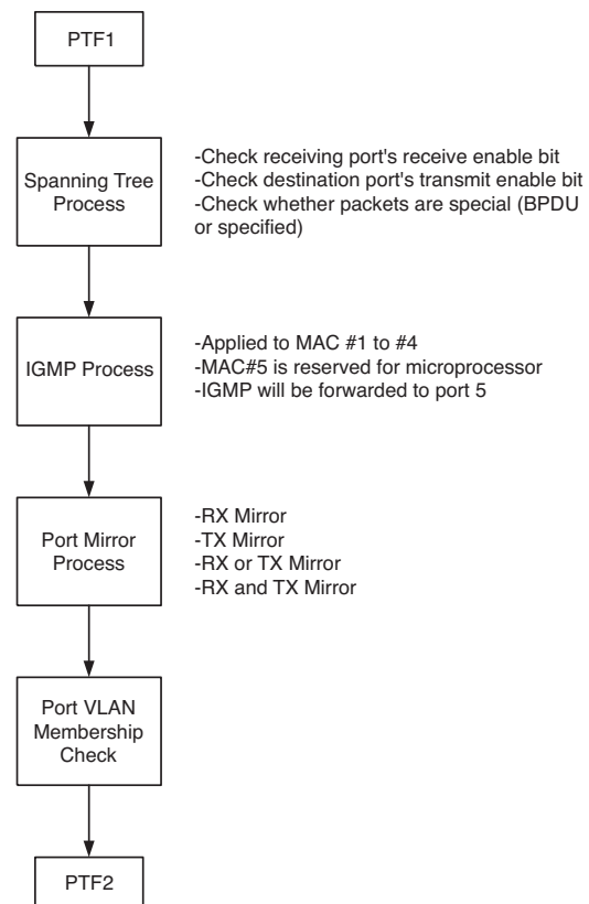
Figure 6. DA Resolution Flowchart—Stage 2
