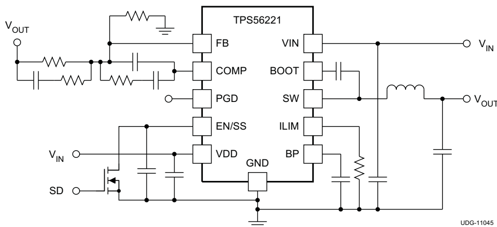
Simplified Application Schematic
