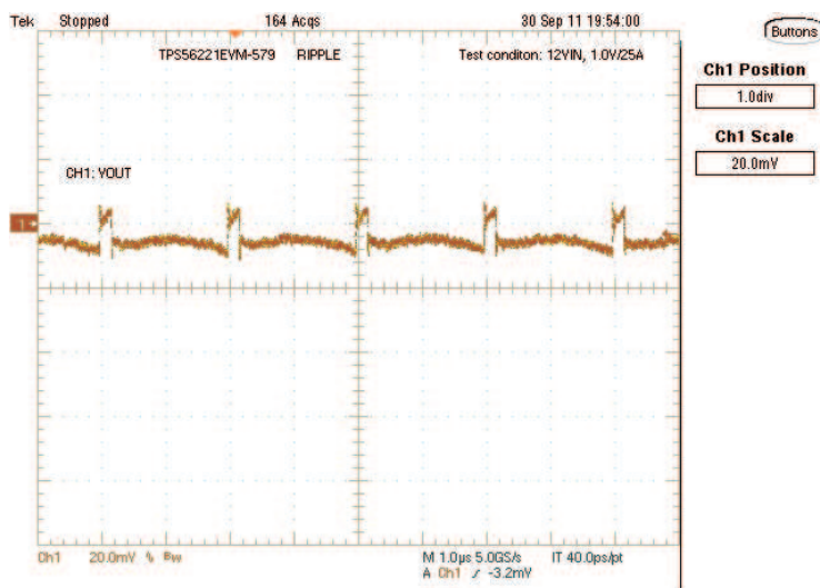
Figure 23. TPS56221 Design Example Output Ripple 20 mV/div, 1.0 \mu\text{s} /div, 20 MHz Bandwidth, AC Coupled
